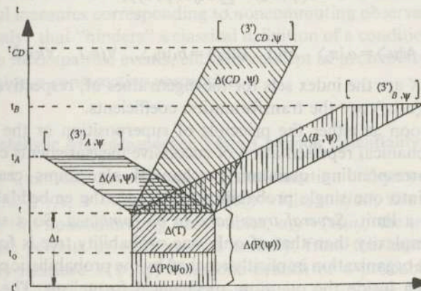
Fig. 1. A quantum mechanical probability tree \mathcal{F}(P(\psi_0), |\psi\rangle) .
